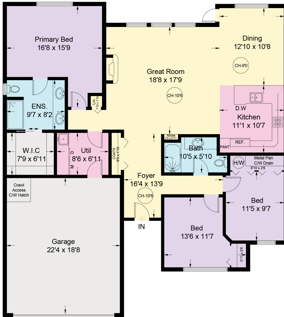
Main Floor - 1640 sq ft
